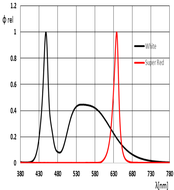
Fig 2. 相对发光光谱 / Relative Spectral Power Distribution vs. Wavelength
